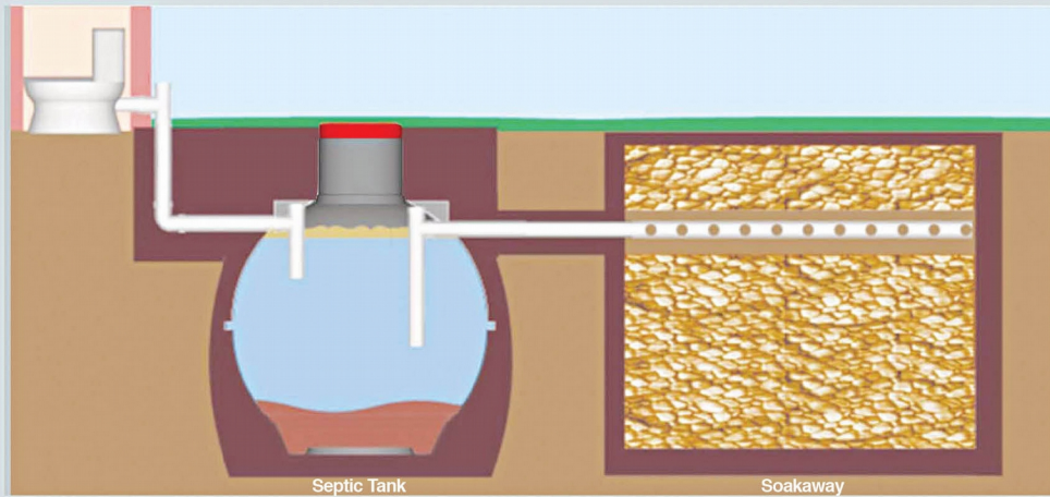
600 Gallons (2,270L) Internal view of septic tank installed
