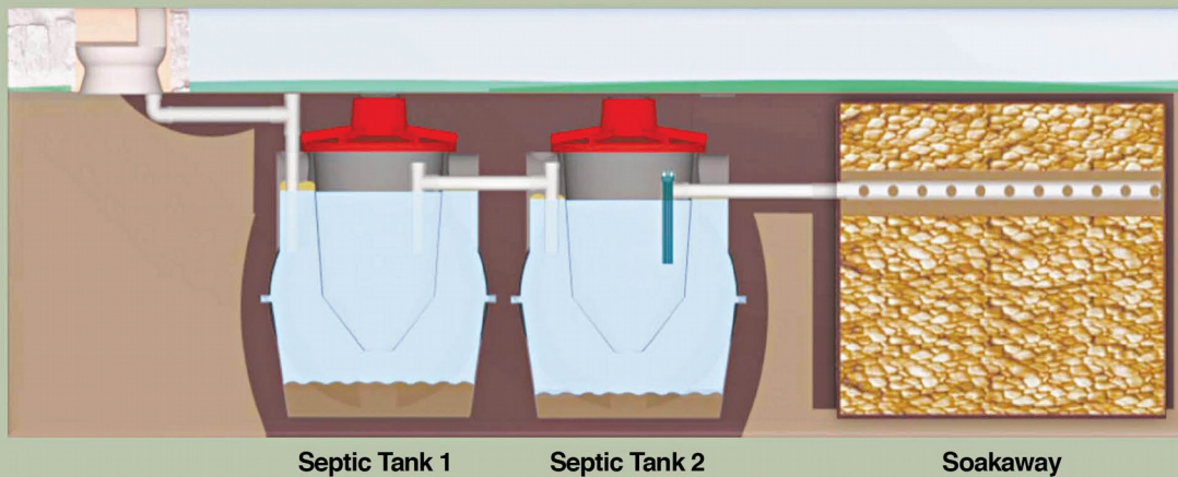
Two Tank System Internal view of two 600 gallon tanks joined to create a larger system
