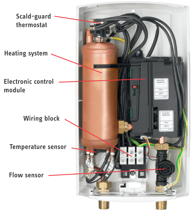
Copper heating element - exclusive to Stiebel Eltron!
